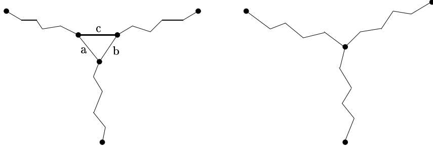
Figure 1: Geodesic triangles in plain groups
