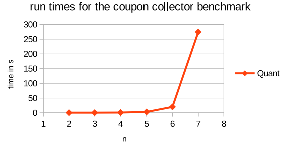
run times for the coupon collector benchmark
