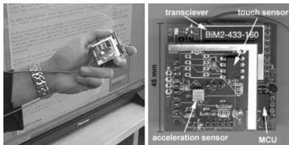
Figure 5: The Pendle hardware is based on two modules. The base board contains processor, memory and radio, and the sensor board touch and acceleration sensors for physical interaction.
