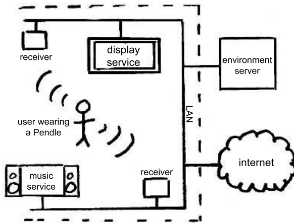
Figure 6: Testbed architecture
